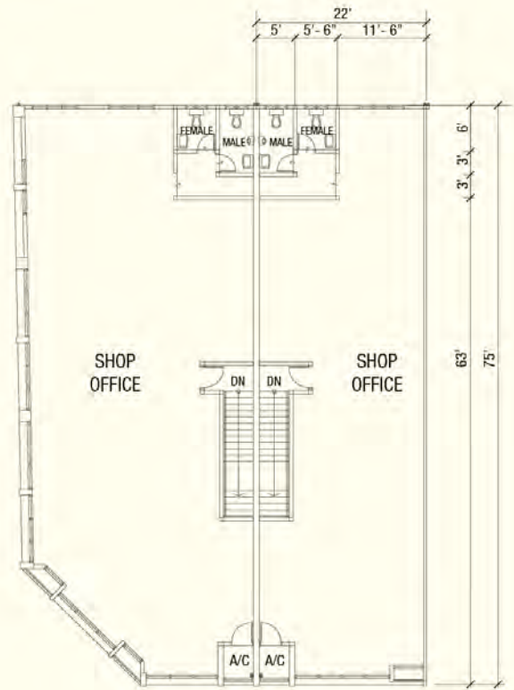
First Floor 一楼
