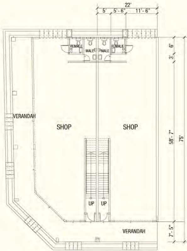
Ground Floor 底楼
